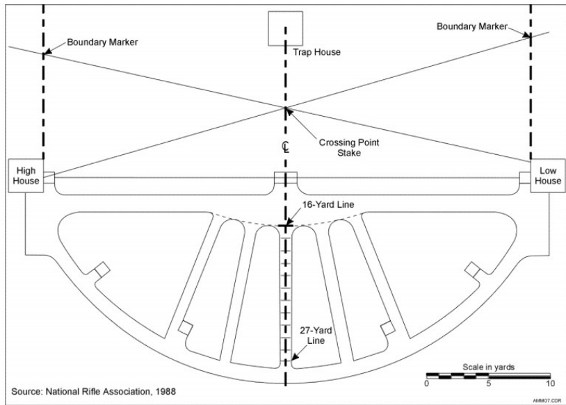
Main features of an example combined trap and skeet range
